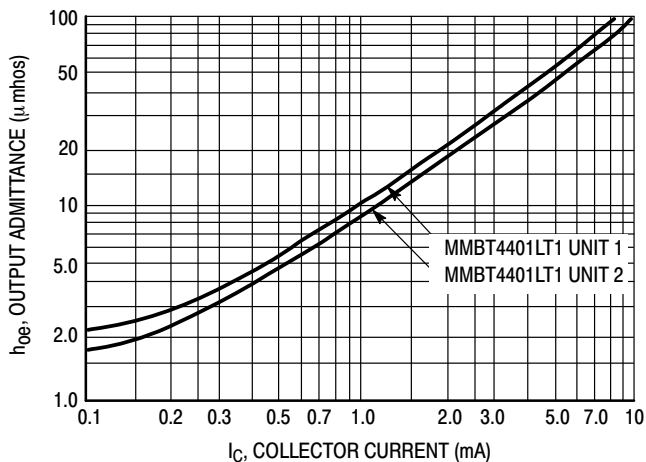
Figure 12. Output Admittance
